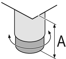
Fig. 10 The adjustable foot can be adjusted from A = 150 \text{ mm} (6 5/16 in) to 180 \text{ mm} (7 1/16 in).*
